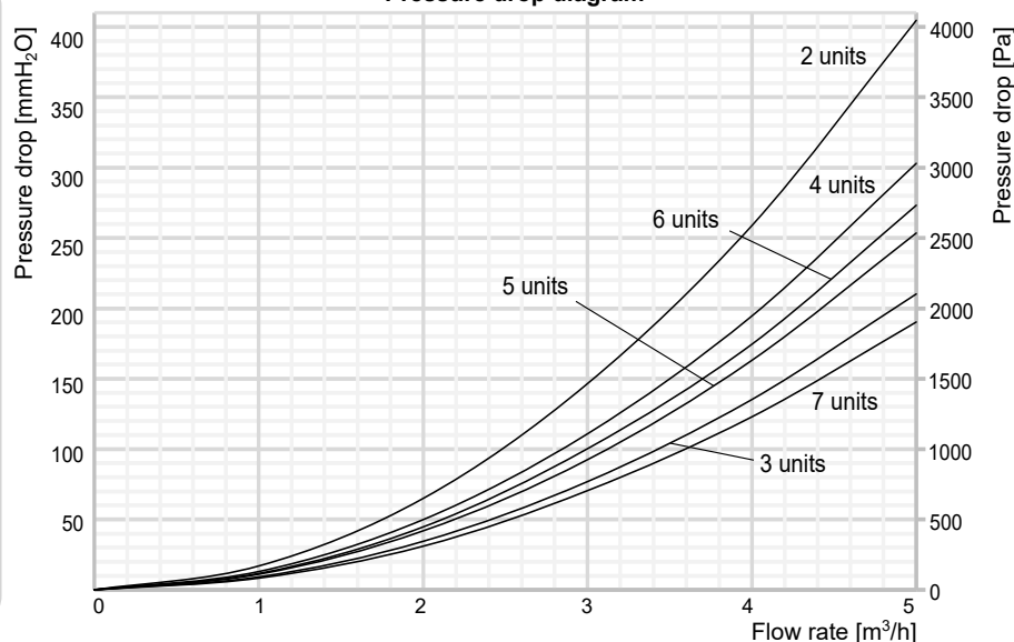
Pressure drop diagram
